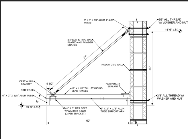
HOLLOW CMU WALL
