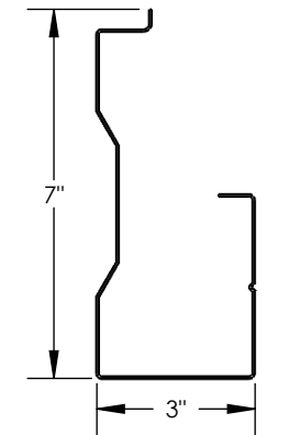
3" x 7" Gutter Fascia
