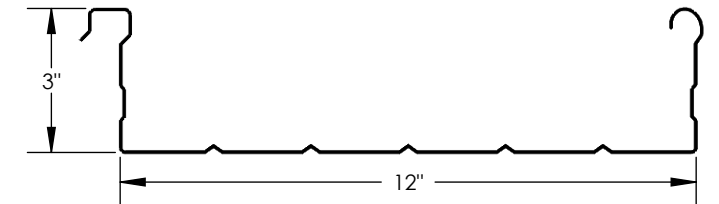
3" x 12" Deck Pan
